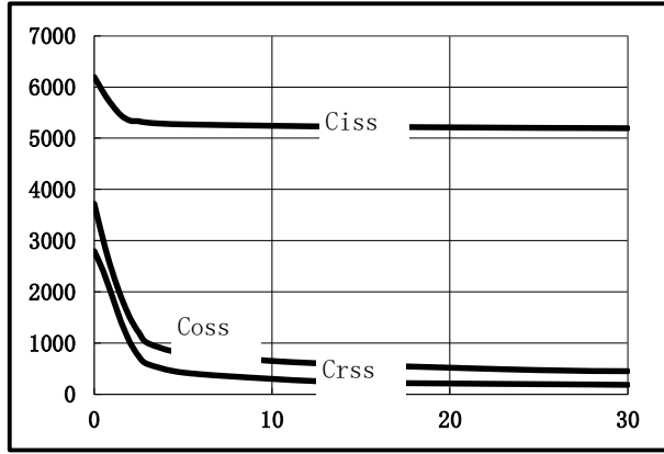
Fig.2 Capacitance Characteristics
