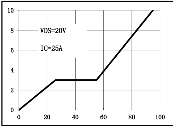
Fig.1 Gate-Charge Characteristics
